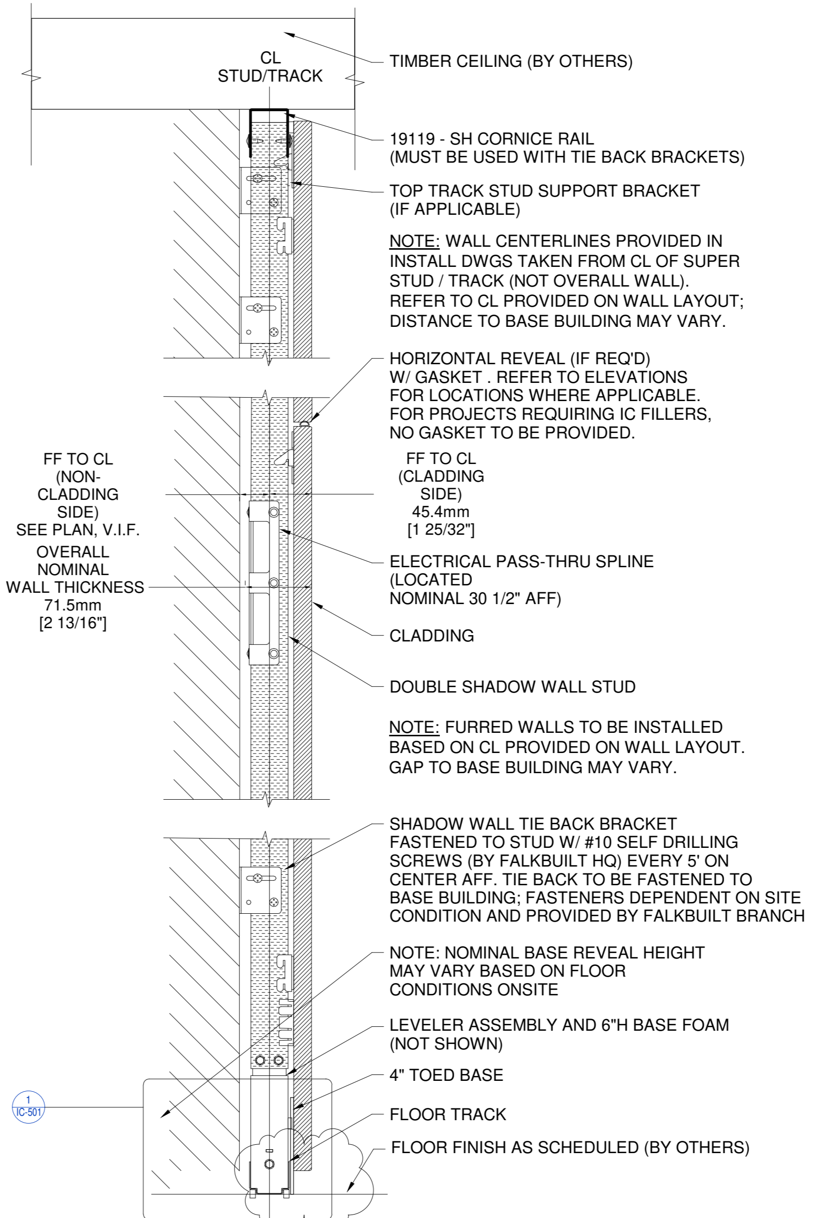
WALL SECTION - SHADOW FURRED WALL CORNICE CEILING W STANDARD BASE REVEAL 3" = 1'-0"
